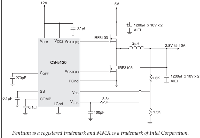
Figure 1: 5V to 3.3V/10A converter.
