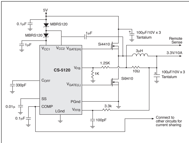
Figure 2: 5V to 3.3V/10A converter with current sharing.
