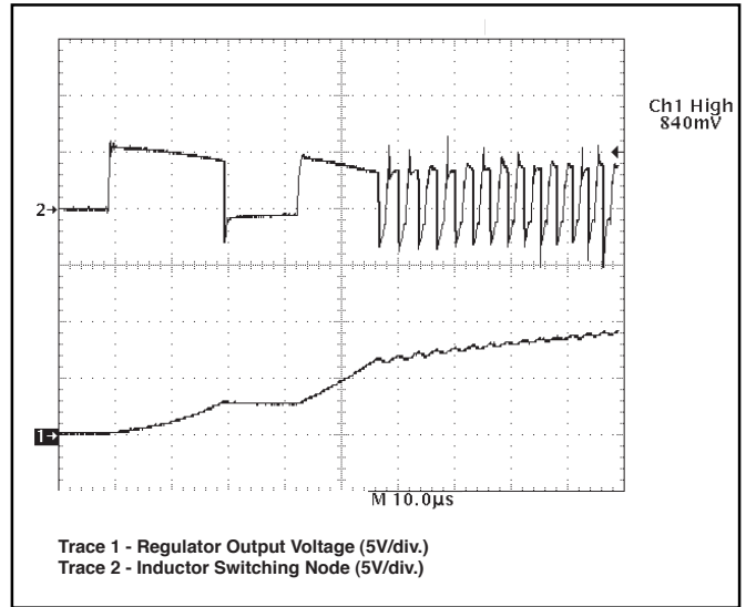
Figure 4: CS-5120 enable startup waveforms.
