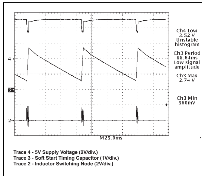
Figure 10: CS-5120 hiccup mode short circuit protection. Gate pulses are delivered while the soft start capacitor charges, and cease during discharge.
