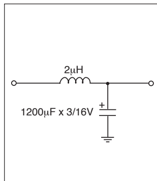
Figure 19: Input Filter
