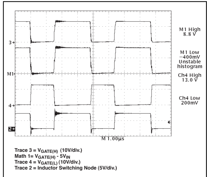
Figure 17: CS-5120 gate drive waveforms depicting rail to rail swing.
