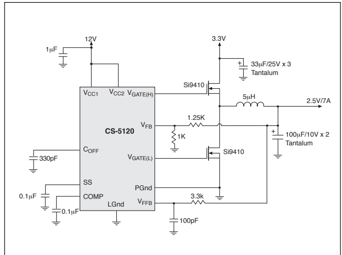
Figure 4: 3.3V to 2.5V/7A converter with 12V bias.
