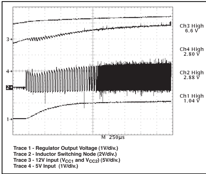
Figure 2: CS-5120 startup in response to increasing V_{CC1} + V_{CC2} input voltages. Extended off time is followed by normal off time operation when output voltage achieves regulation to the error amplifier output.
