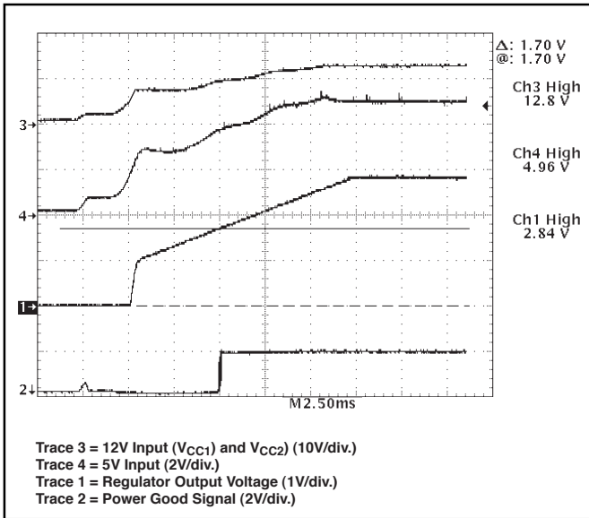
Figure 16: CS-5120 during power up. Power Good signal is activated when output voltage reaches 1.70V.
