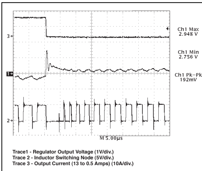
Figure 9: CS-5120 response to 13A load turn off (output set for 2.8V). V^2 control topology immediately connects inductor to ground, providing 0% duty cycle. Regulation is achieved in less than 10\mu\text{s} .
