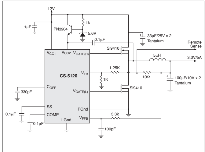
Figure 3: 12V to 3.3V/5A converter with remote sense.
