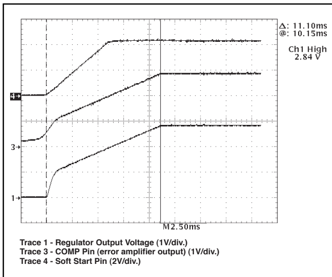
Figure 3: CS-5120 startup waveforms.
