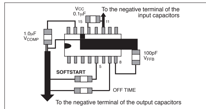
Figure 20: Layout Guidelines
